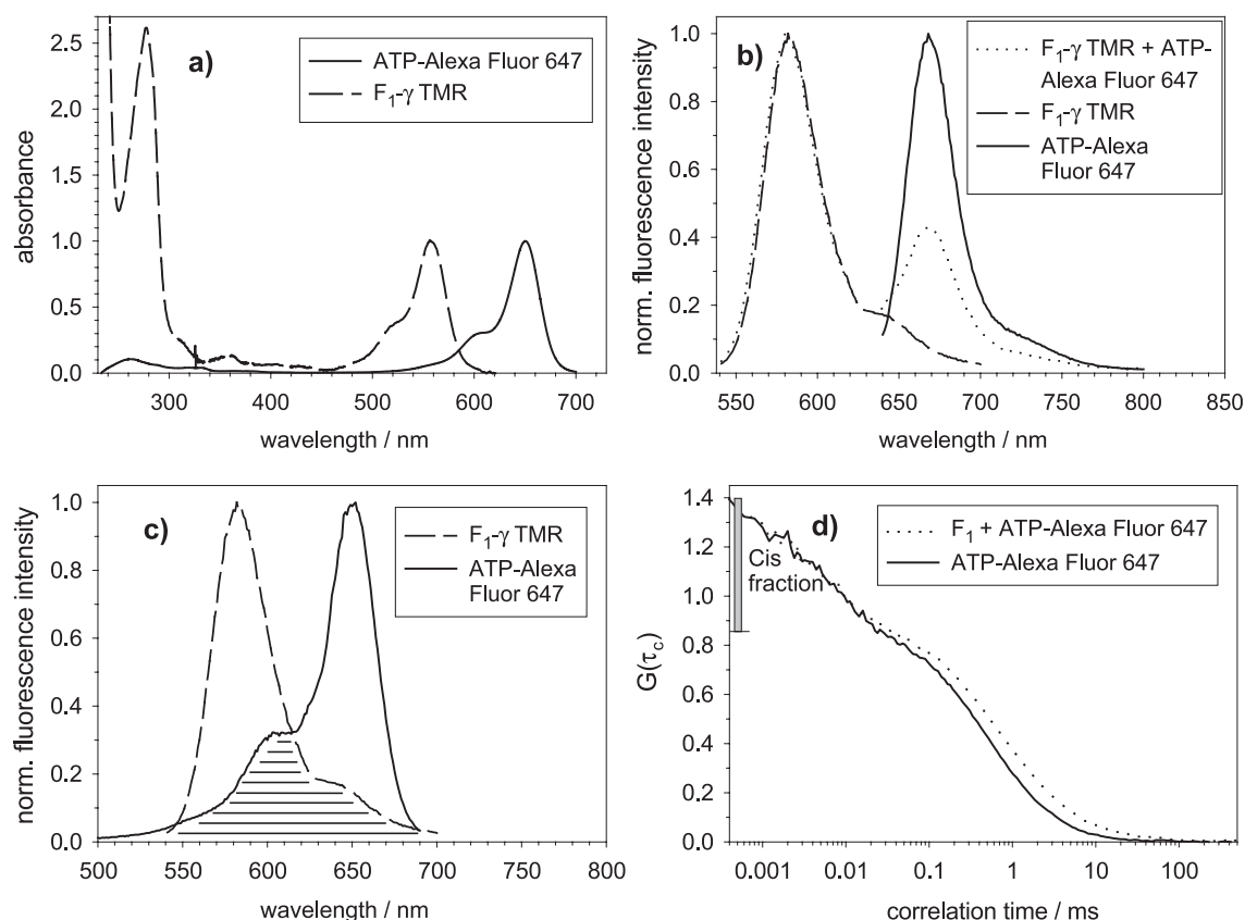
Fig. 2. (a) UV-VIS absorbance spectra of F 1 -γTMR-ATPase (1.5 μM) and ATP-Alexa Fluor 647 (2.4 μM) in buffer A. (b) Normalised fluorescence emission spectra of F 1 -γTMR-ATPase (200 nM, excited at 532 nm), ATP-Alexa Fluor 647 bound to F 1 -γTMR-ATPase (200 nM, excited at 532 nm) and free ATP-Alexa Fluor 647 (800 nM, excited at 632 nm) in buffer A. (c) Normalised emission spectrum of F 1 -γTMR-ATPase (200 nM, excited at 532 nm) and absorbance spectrum of ATP-Alexa Fluor 647 (2.4 μM). Spectral overlap of these two curves is shown in the diagram (dashed area). (d) Fluorescence autocorrelation of free ATP-Alexa Fluor 647 and ATP-Alexa Fluor 647 bound to F 1 . The two correlation functions G(\tau_c) show different translational diffusion correlation times. In addition below correlation times of 100 μs, a relaxation process can be seen which is due to a photo-induced cis – trans -isomerisation within in the ATP-Alexa Fluor 647 dye. Approximately 40% of the fluorophores are in the non-fluorescent cis -conformation.
